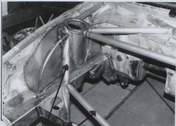
Engine mountings
