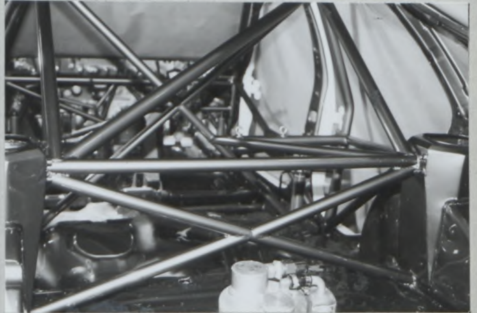
PHOTO No. 8 (REAR SUPPORT BARS TO STRUT TOWER)
